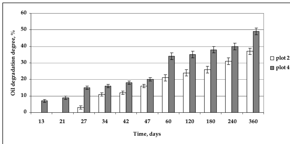
Fig. 10. Oil removal in the pilot field experiment
