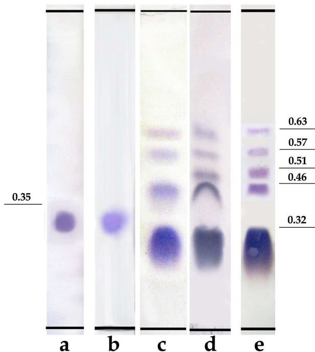
Fig. 5. Chromatograms of purified samples of biosurfactants synthesized by microorganisms ( R_f is shown): a) Pseudomonas fluorescens 142NF (pNF142); b) Pseudomonas putida BS3701 (pBS1141, pBS1142); c) Rhodococcus sp. S67; d) Rhodococcus sp. X5; e) Rhodococcus sp. 26
