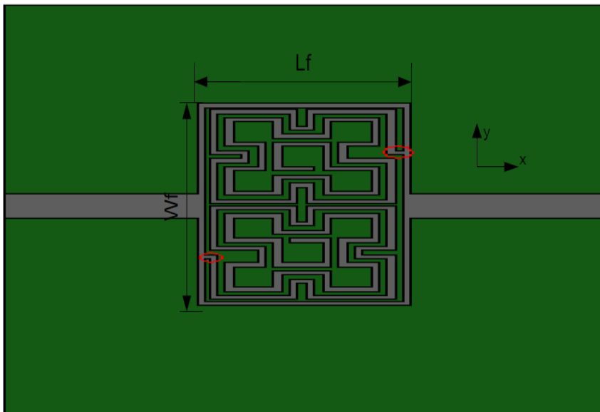
Fig. 8. Fractal spiral resonator based band-stop filter
