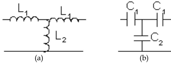
Fig. 3. Equivalent circuit model of one unit cell of (a) negative permittivity and (b) negative permeability materials
