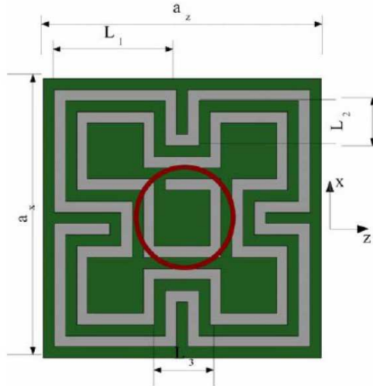
Fig. 5. Fractal spiral resonator geometry
