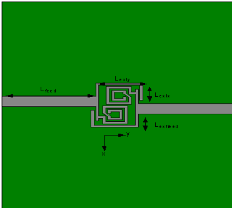
Fig. 12. Thin wire loaded spiral resonator based BPF
