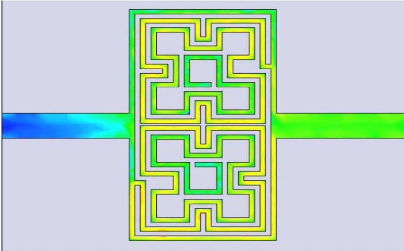
Fig. 10. Surface current distribution of fractal spiral resonator based BSF at 1.38GHz
