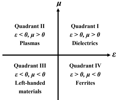
Fig. 1. Permittivity-permeability diagram
