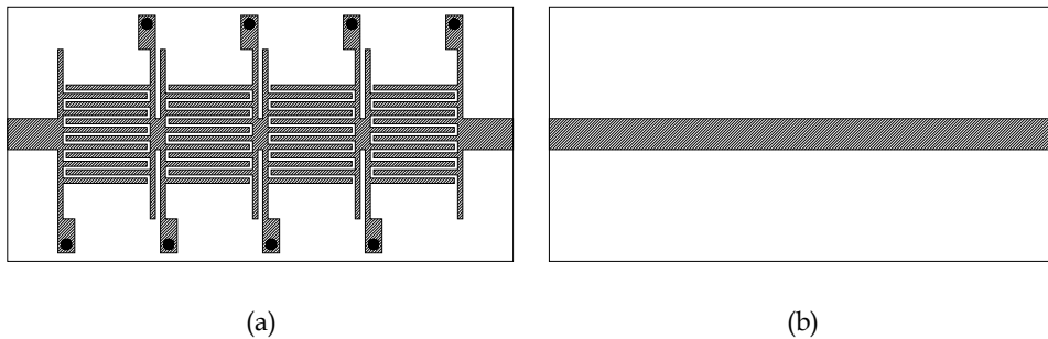
Fig. 9. TTDs using (a) four CRLH TL unit cells and (b) RH TL
