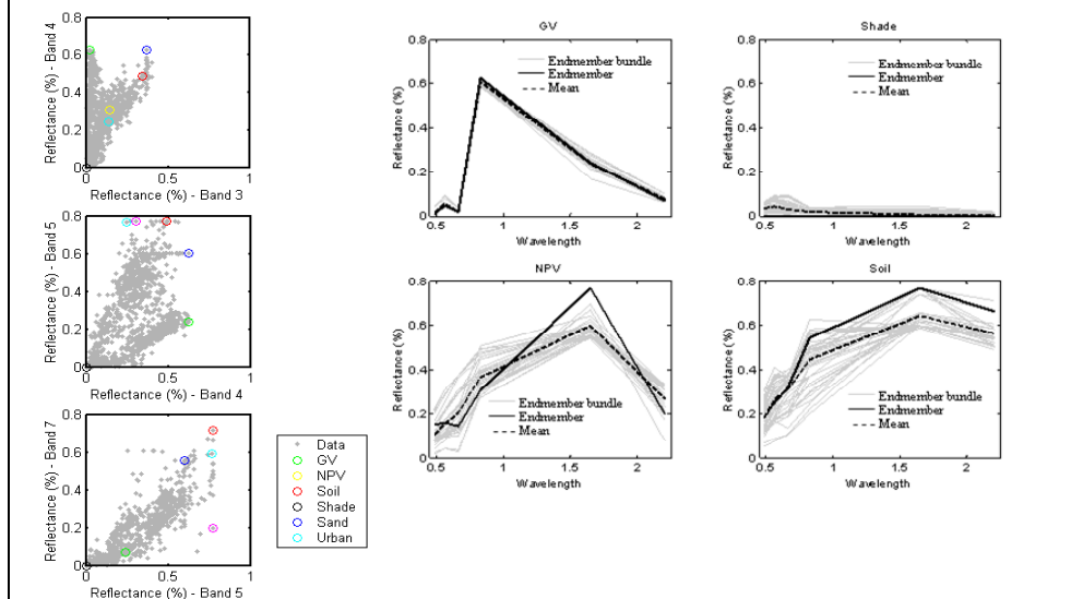
Fig. 3. Image scatter-plots of Landsat bands in reflectance space and the spectral curves of GV, Shade, NPV and Soil (source: Souza Jr. et al., 2005).
