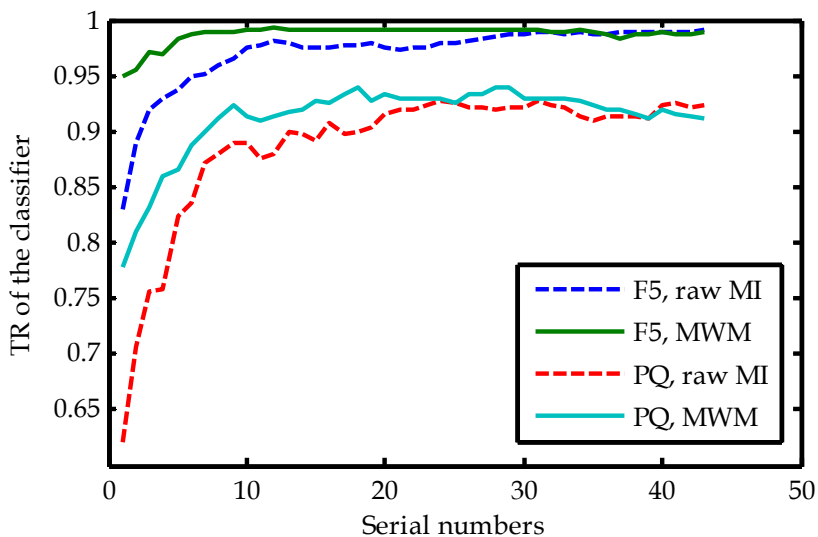
Fig. 8. Comparison of the performance between the classifier using WMW values (solid lines) and the raw MI values (dotted lines) for feature selection, with embedding rate 0.15bpac.
