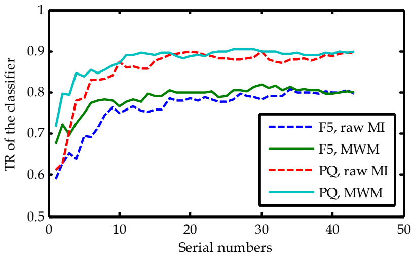
Fig. 6. Comparison of the performance between the classifier using WMW values (solid lines) and the raw MI values (dotted lines) for feature selection, with embedding rate 0.05bpac.
