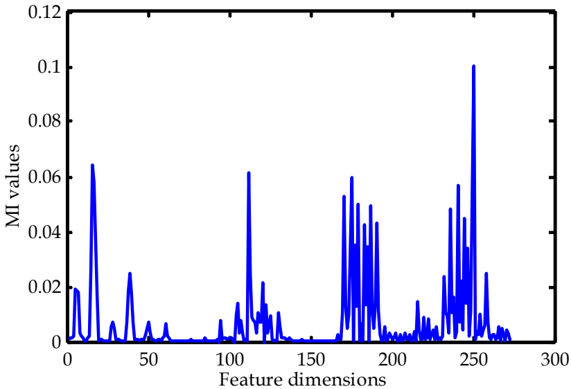
Fig. 2. MI values of Merging Markov and DCT features
