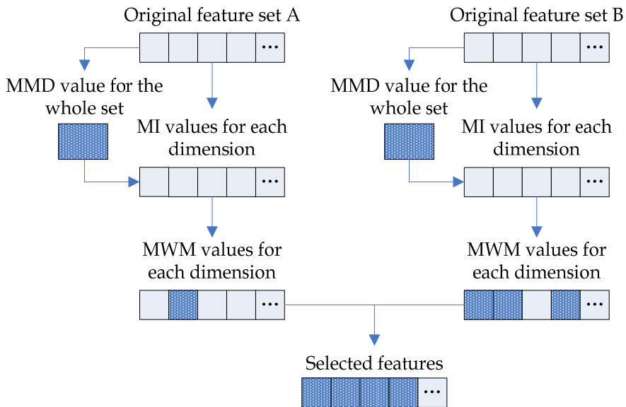
Fig. 5. Overview of the MWM feature selection
