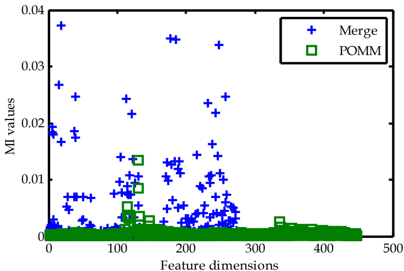
Fig. 3. Comparison of MI values between the Merging Markov and DCT features ('Merge', cross marked ones) and the Partially Ordered Markov Model features ('POMM', square marked ones)
