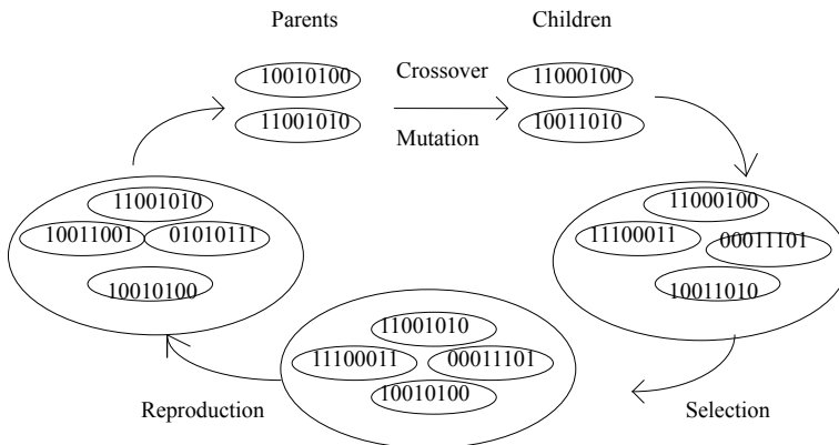
Fig. 2. Flow chart of genetic algorithm
