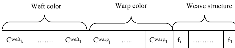
Fig. 5. Representation Scheme of Chromosome
