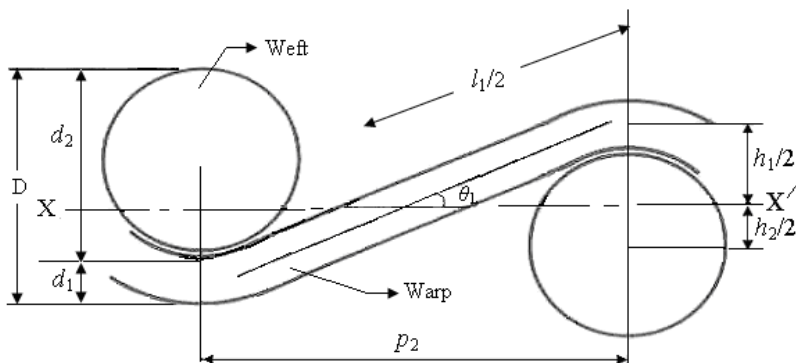
Fig. 5. Peirce's model of plain weave
