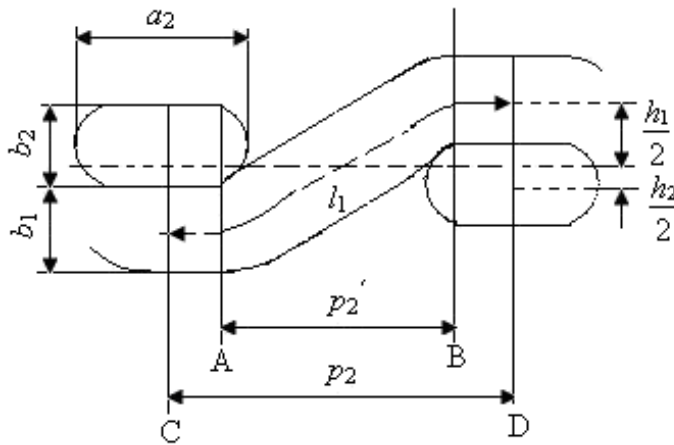
Fig. 8. Race track cross-section
