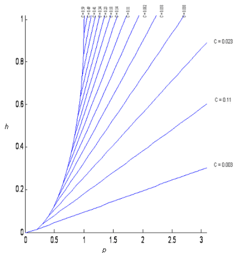
Fig. 9. Relation between thread spacing and crimp height
