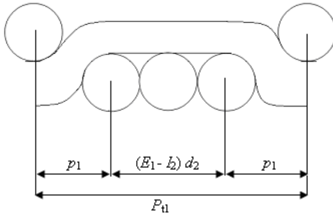
Fig. 14. Jammed structure for 1/3 weave (circular cross-section along warp)
