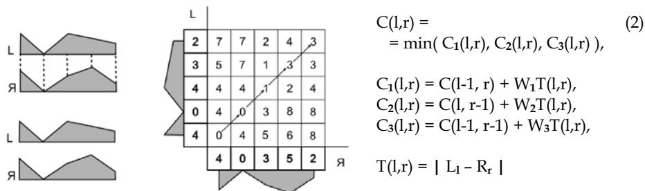
Figure 4. Right: Error measures that are used for Dynamic Programming. Centre: Symmetric patterns' search space including costs and corresponding mapping path ( W_i = 1 ). Left: Resulting (linear) correspondences
