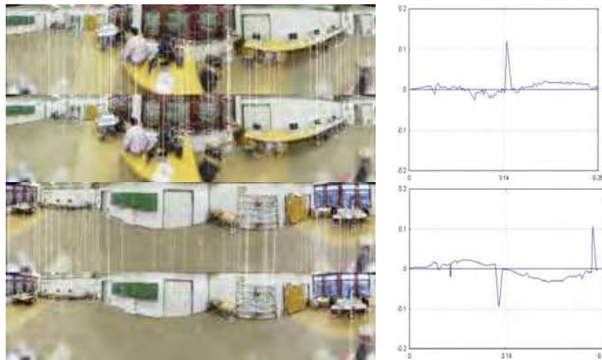
Figure 12. Top: Between images 122 and 123. The algorithm computes d(\alpha) = -215 , c_1(\alpha) = c_2(\alpha) = 0 and correctly returns “No move”. Bottom: Between images 24 and 25. The algorithm computes d(\alpha) = -428 , c_1(\alpha) = -95 , c_2(\alpha) = 95 and returns “Move in direction 340°”
