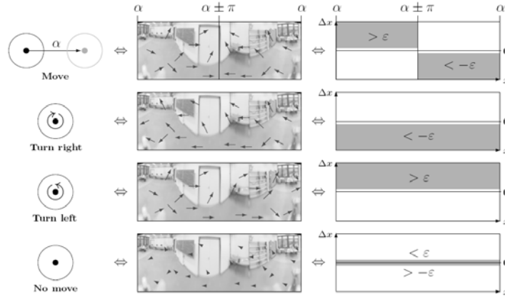
Figure 11. The four basic movements “Move \alpha ”, “Turn right”, “Turn left”, and “No move”. Typical feature shifts for those movements are shown in the centre column. On the right column, the corresponding homography sectors are depicted, e.g. a “Turn right” action is to result in feature shifts in negative x-direction only
