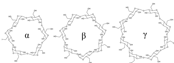
Fig. 5. Chemical structure of the cyclodextrins
