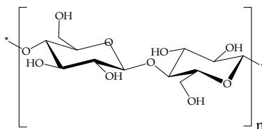
Fig. 6. Chemical structure of the cellulose
