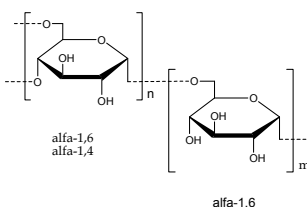
Fig. 3. Chemical structure of the dextran
