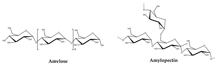
Fig. 1. Chemical structure of the starch
