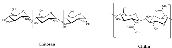
Fig. 2. Chemical structure of the chitosan and chitin
