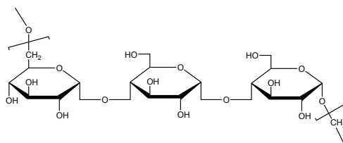
Fig. 4. Chemical structure of the pullulan
