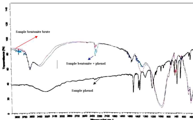
Fig. 3. Spectra FTIR of the studied samples
