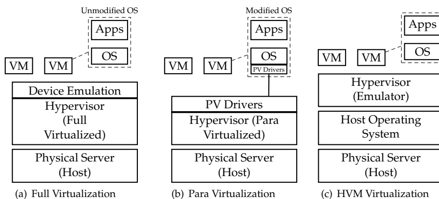
Fig. 3. Virtualization approaches.
