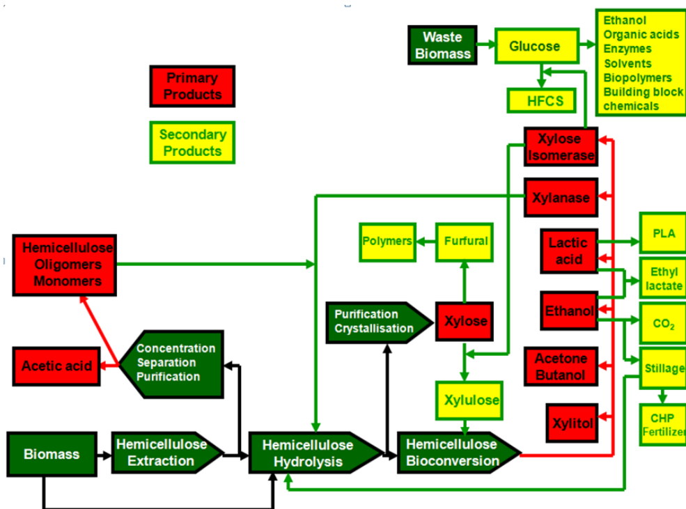
Fig. 8. Schematic of a hemicellulose-based biorefinery
