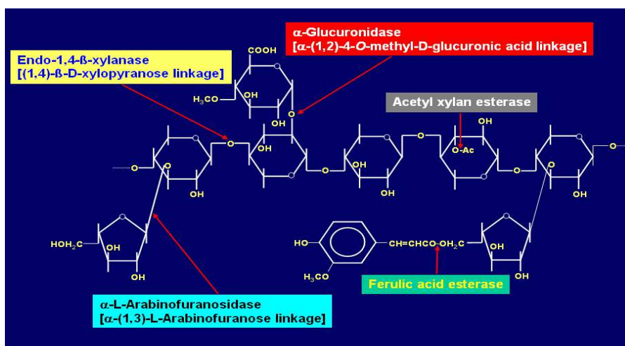
Fig. 3. Enzymatic hydrolysis of xylan
