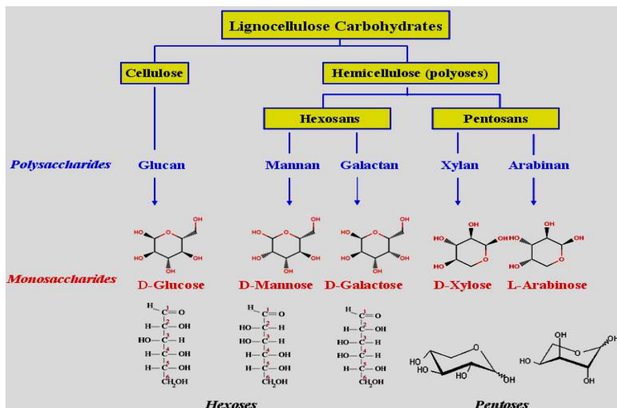
Fig. 2. Chemical structure of lignocellulose carbohydrates
