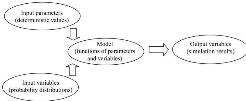
Fig. 3. Elements of the Monte Carlo simulation
