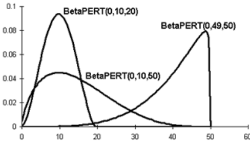
Fig. 6. Examples of BetaPERT distributions
