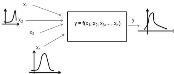
Fig. 2. Monte Carlo simulation
