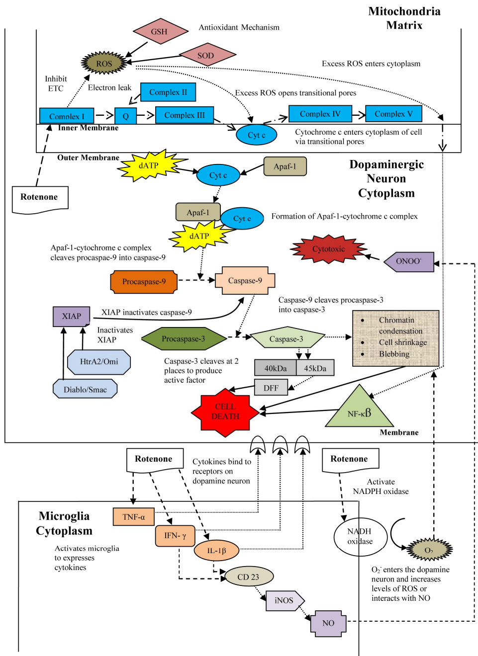
Fig. 1. Mechanism of action of rotenone
