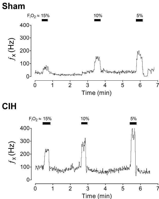
Fig. 1. Carotid body chemosensory potentiation induced by intermittent hypoxia in the rat. The carotid chemosensory discharges in response to various levels of inspired O_2 ( F_iO_2 \sim 15 to 5%) were measured from the carotid sinus nerve of a sham rat exposed to air to air cycles and a rat exposed to chronic intermittent hypoxia (CIH) for 21 days. f_x , frequency of carotid chemosensory discharges, expressed in Hz.
