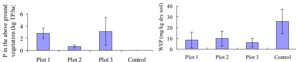
Fig. 9. P content of above ground vegetation and soil WEP in the study plots and control in the Glennamong
