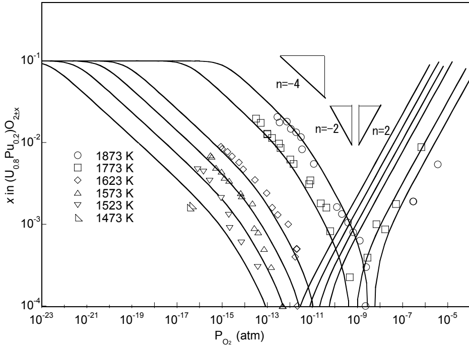
Fig. 5. The P_{O_2} versus x in (U_{0.8}Pu_{0.2})O_{2\pm x}
