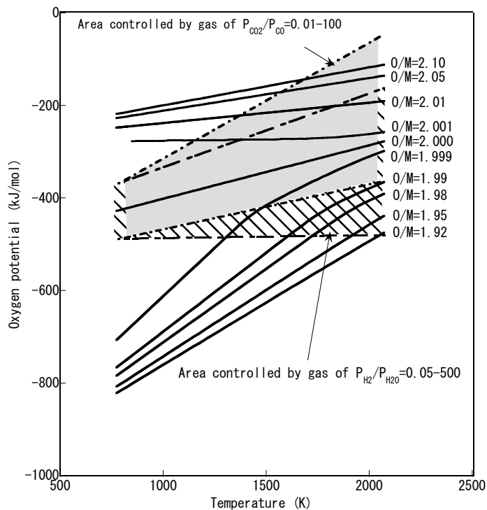
Fig. 3. Oxygen potential of (U_{0.8}Pu_{0.2})O_{2\pm x}
