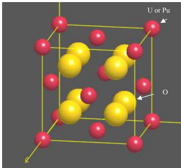
Fig. 1. CaF_2 type fluorite structure
