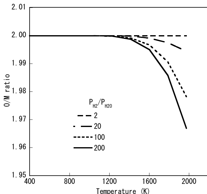
Fig. 7. O/M variation of (U_{0.8}Pu_{0.2})O_{2\pm x} as a function of P_{H_2} / P_{H_2O}
