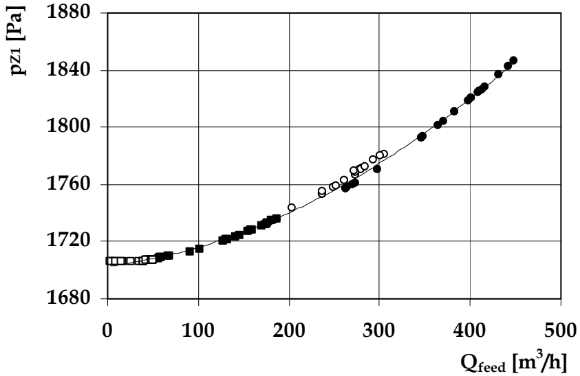
Fig. 9. The effect of gas stream size feeding the network Q_{feed} on the gas stream overpressure p_{z1} ; (●) t = -16\text{ }^{\circ}\text{C} , (○) t = -4\text{ }^{\circ}\text{C} , (■) t = 8\text{ }^{\circ}\text{C} , (□) t \geq 18\text{ }^{\circ}\text{C} .
