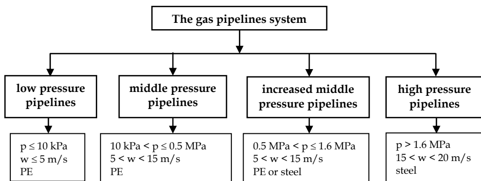
Fig. 2. The main types of gas pipeline networks.
