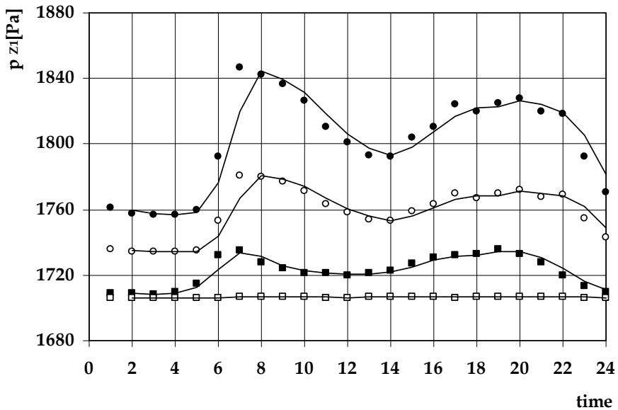
Fig. 10. The change of the gas stream overpressure p_{z1} feeding the network in particular hours of the day; various values of air temperature; (●) t = -16\text{ }^{\circ}\text{C} , (○) t = -4\text{ }^{\circ}\text{C} , (■) t = 8\text{ }^{\circ}\text{C} , (□) t \geq 18\text{ }^{\circ}\text{C} .
