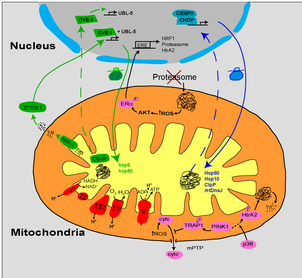
Fig. 2. Mitochondrial stress signalling
