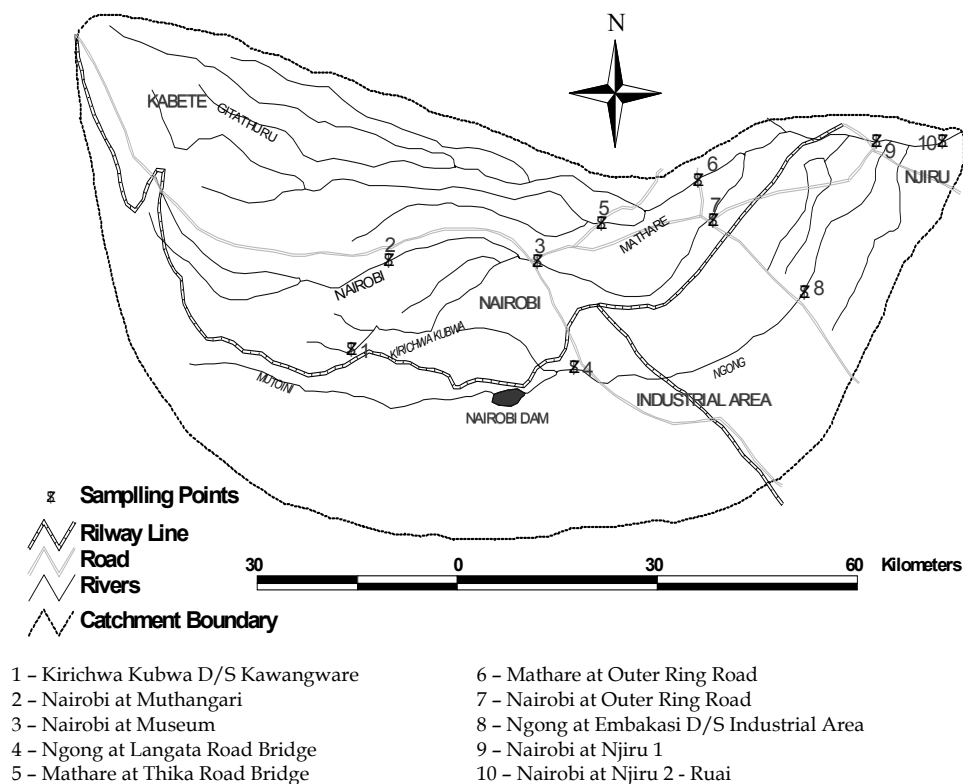
Fig. 1. Distribution of study sampling points (1999-2002)
