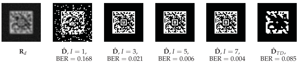
Fig. 25. The example of the QR code restoration by the distributed IDN marginalizing at the symbol block level with bias state variables (Pd-SyD, 2 nd version): Kernel A_{GBC, 2/10}, N_b = 8, \Delta_Q = 3, C = 612, \mu_T = 50, \mu_R = 25, \sigma_R = 10 .
