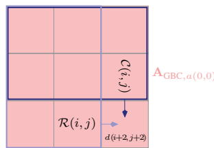
Fig. 12. The primary layout of auxiliary state variables \mathcal{R}(i, j) and \mathcal{C}(i, j) for the ISI channel \mathcal{A}_{\text{GBC}, a(0,0)} .
