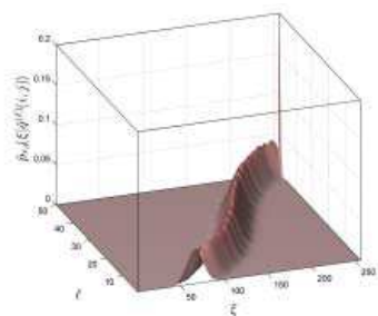
(b) The PDF for the blurring channel A_{GBC,3/10} : C = 542 , \mu_T = 150 , \mu_R = 40 , \sigma_R = 25 .
