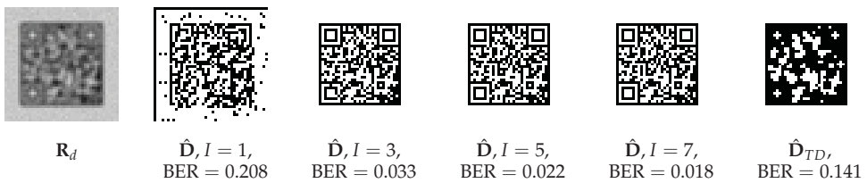
Fig. 24. The example of the QR code restoration by the distributed IDN marginalizing at the symbol block level with bias state variables (Pd-SyD, 1 st version): Kernel A_{GBC, 2/10}, N_b = 8, \Delta_Q = 3, C = 612, \mu_T = 50, \mu_R = 25, \sigma_R = 10 .
