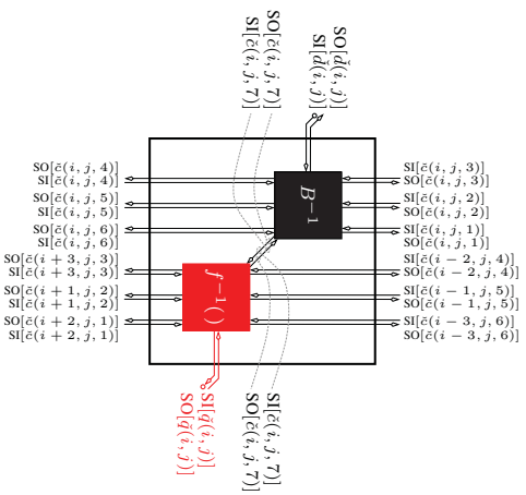
(c) The IDN cell in the node (i, j) .
