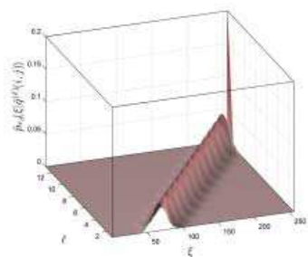
(f) The PDF for the blurring channel A_{BOM,\pi/4} : C = 542 , \mu_T = 150 , \mu_R = 40 , \sigma_R = 25 .
