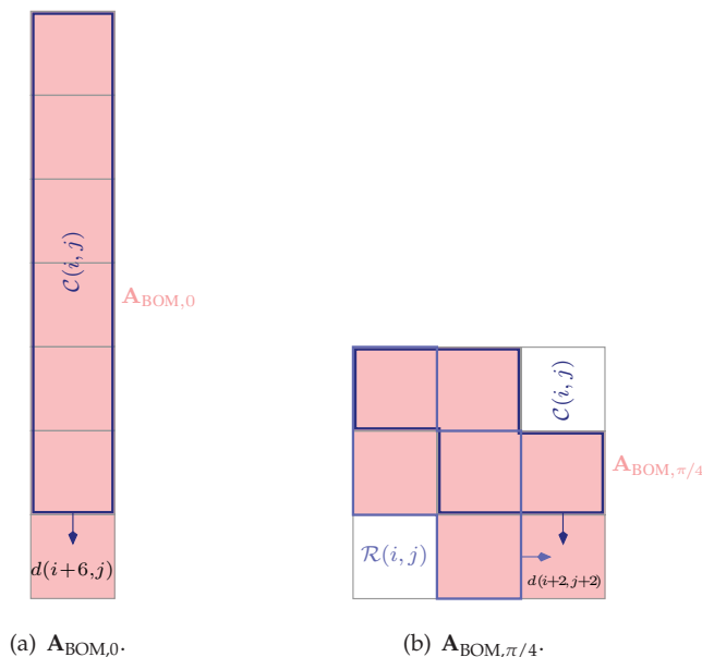
Fig. 28. The shapes of auxiliary state variables \mathcal{R}(i, j) and \mathcal{C}(i, j) in the IDN marginalizing at the symbol block level for the ISI channel \mathbf{A}_{BOM,\varphi} .
