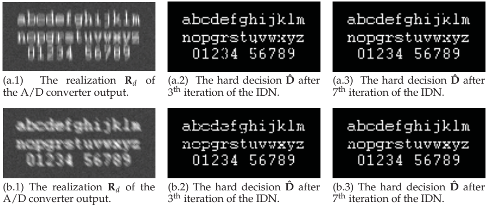
Fig. 31. The examples of image restorations by the distributed IDN marginalizing at the symbol level (Pd-PgD) for the channels A_{BOM,0}(a) and A_{BOM,\pi/4}(b) merged with the simple noise model including the thermal noise and the quantization noise: N_b = 8, \Delta_Q = 3, C = 768, \mu_T = 200 .
