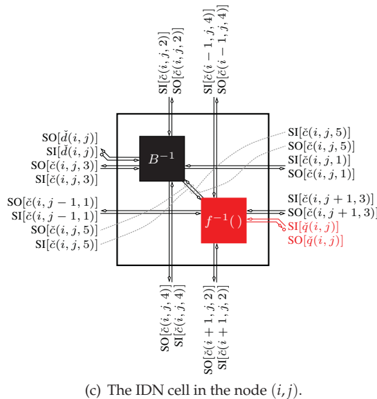
Fig. 23. The EN and IDN marginalizing at the symbol level with the centered topology for the ISI channel \mathbf{A}_{\text{SIBC},d}(0,0) .
