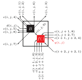
(b) The EN cell in the node (i, j) .
