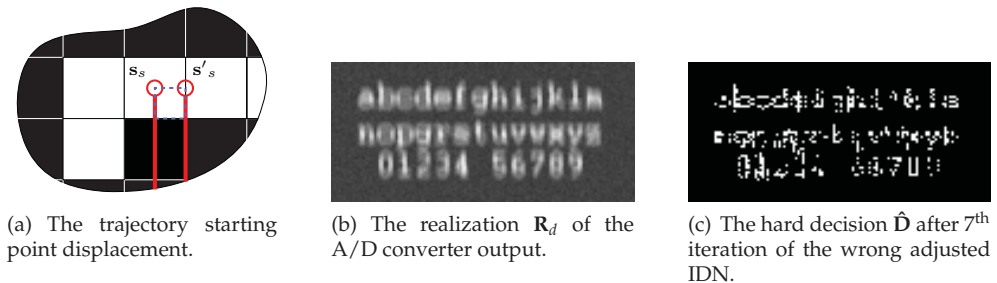
Fig. 32. The example of the wrong image restoration by the distributed IDN marginalizing at the symbol level (Pd-PgD), that was incorrectly set by the A_{BOM,0} at the true blurring A'_{BOM,0} merged with the simple noise model including the thermal noise and the quantization noise: C = 768, N_b = 8, \Delta_d = 3, \mu_T = 200 .
