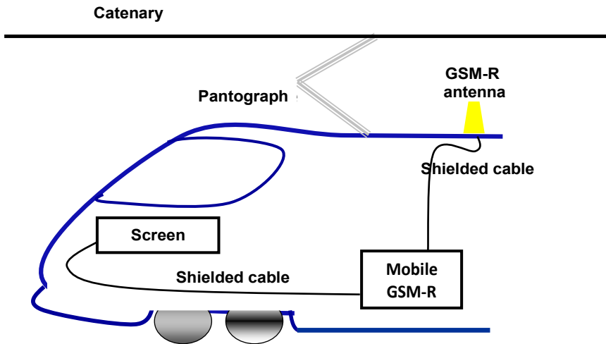
Fig. 2. Illustration of the on-board GSM-R system
