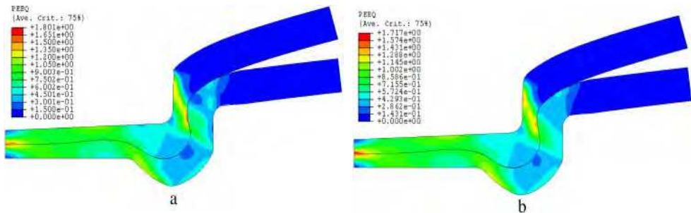
Fig. 16. Equivalent plastic strain distribution (Oudjene et al., 2009): (a) without remeshing and (b) with remeshing.
