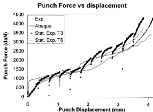
Fig. 14. Computed punch force variation (Hamel et al., 2000).
