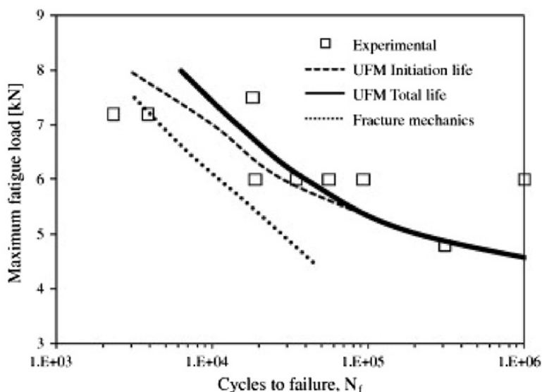
Fig. 22. Extended L–N curves using UFM and fracture mechanics (Shenoy et al., 2010).
