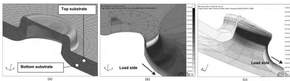
Fig. 15. FEA of clinched joints (Carboni et al., 2006): (a) brick modelling of an indentation point, (b) max principal stress in the bottom substrate and (c) maximum Von Mises stress around the neck of the indentation point.
