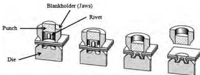
Fig. 1. SPR operation with a semi-tubular rivet.
