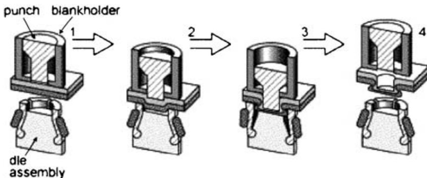
Fig. 10. Principle of clinching with a round tool.
