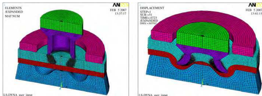
Fig. 6. Initial and final configuration of the joint (Casalino et al., 2008).
