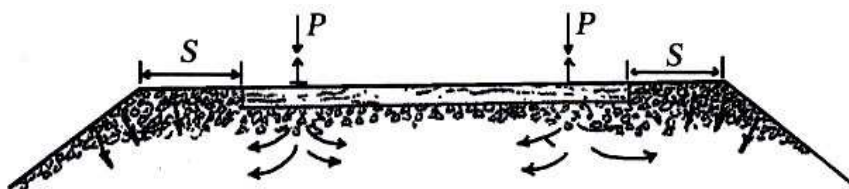
Fig. 6. Changing the location of ballast under the load of passing train
