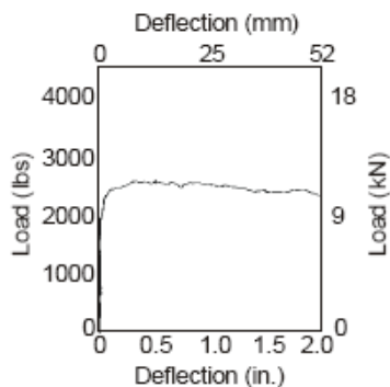
Fig. 11. Post-stabilization and before passing traffic results
