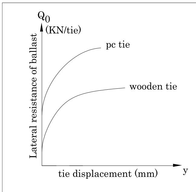
Fig. 3. The relationship between lateral resistances and displacement
