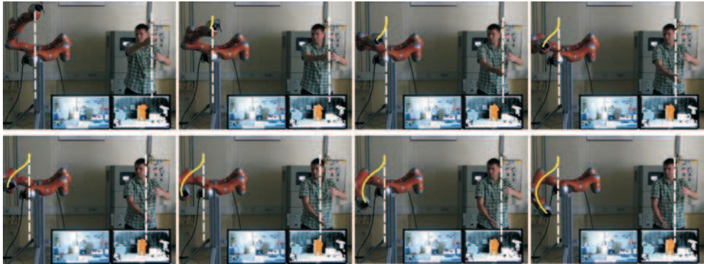
Fig. 16. A sequence of still photographs shows the movement of two Kuka LWR robots, while they successfully avoid each other. The desired movement for the robots is imitated in real time using the Microsoft Kinect sensor for the tracking.
