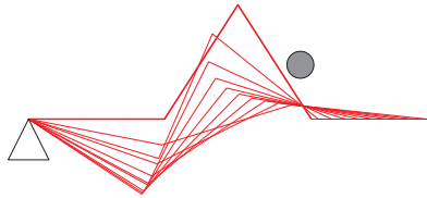
Fig. 2. Planar 3DOF manipulator: tracking of a line and obstacle avoidance using the Jacobian J_{d_o}
