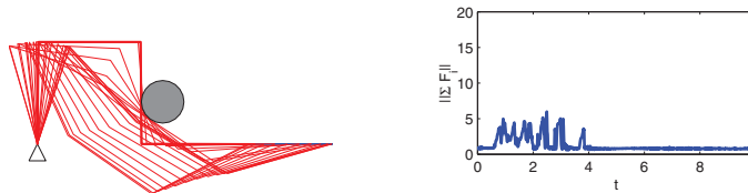
Fig. 18. Planar 4DOF manipulator tracking a circle while and avoiding obstacles using bumper and a virtual forces controller
