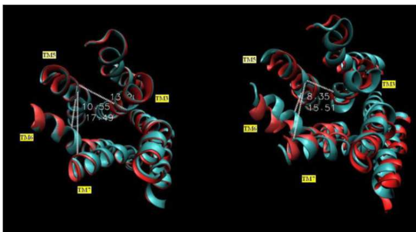
Fig. 4. Movement of TM6 towards TM5 in D 2 model with reduced disulfide bridge.
