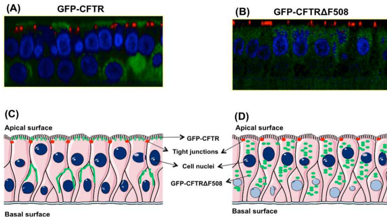
Fig. 2. Cellular localisation of the GFP-CFTR and GFP-CFTR \Delta F508 protein in ex vivo reconstituted human airway epithelium after gene transfer with Ad5-GFP-CFTR (A) and Ad5-GFP-CFTR \Delta F508 (B). (A), (B) : reconstructed images of sagittal sections of transduced epithelia generated from the z-stack images obtained in confocal fluorescence microscopy. (C), (D) : schematic representation of the images shown in (A) and (B), respectively.
