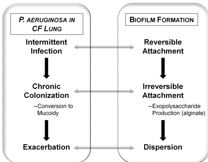
Fig. 2. Similarities between P. aeruginosa colonization of the CF lung and in vitro P. aeruginosa biofilm formation. The transition from reversible to irreversible attachment is mirrored in the transition from intermittent to chronic colonization. Similarly, just as bacteria in mature biofilms secrete exopolysaccharides, the conversion to mucoidy observed with CF isolates signals the overproduction of the exopolysaccharide alginate. Finally, it is possible that bacteria present during an exacerbation could represent bacteria that have dispersed from the biofilm and reverted to the planktonic phenotype expressing acute virulence factors.
