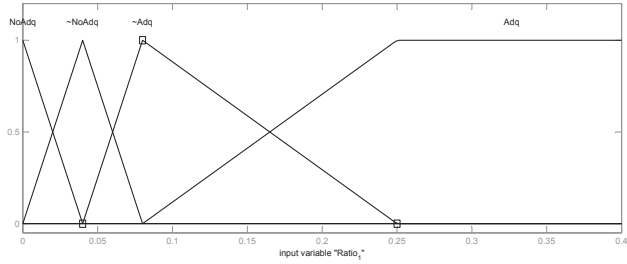
Fig. 9. Membership functions for input variable Ratio_1
