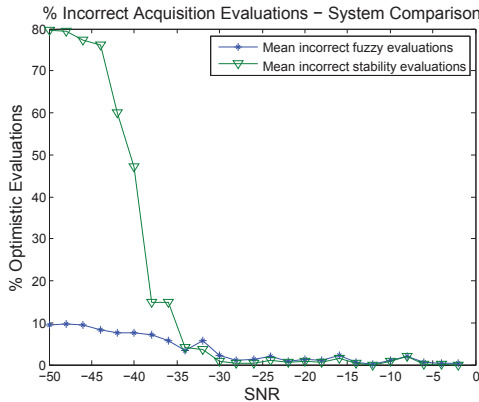
(c) Comparison of the incorrect Optimistic evaluations for Fuzzy and Stability Controls
