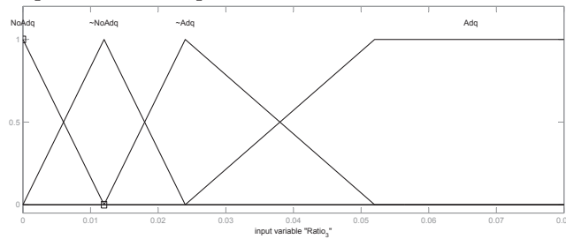
Fig. 11. Membership functions for input variable Ratio_3
