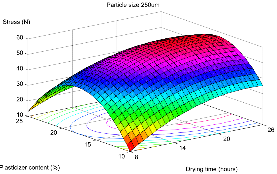
Fig. 4. Response surface of TPCF material with particle size 250 µm
