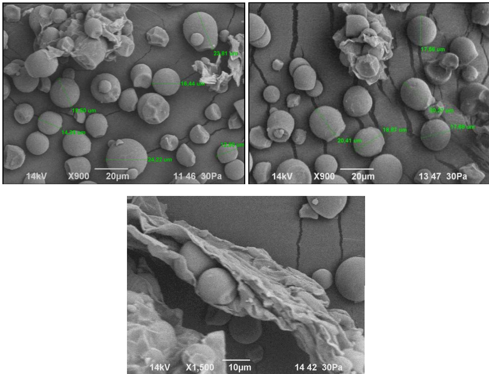
Fig. 2. SEM microphotographs cassava flour
