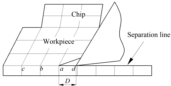
Fig. 3. Geometrical criterion model
