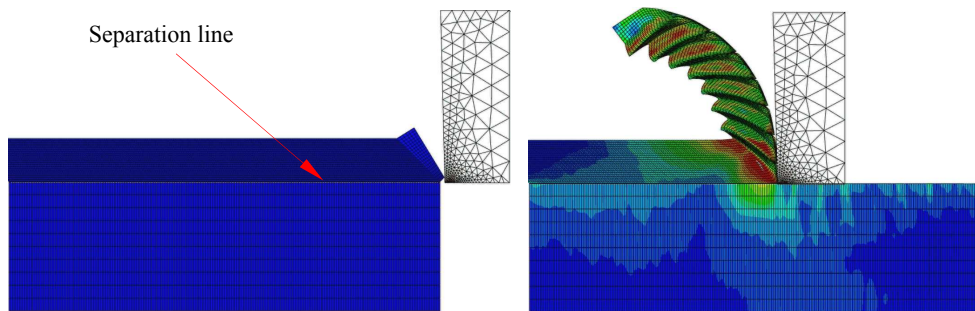
Fig. 4. FE simulation based on geometrical separation criterion
