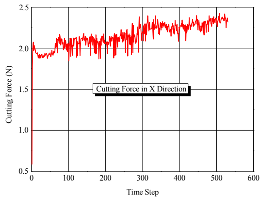
Fig. 7. Simulation results of cutting force
