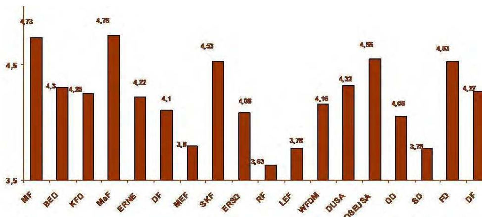
Fig. 8. Oil content of agroecological groups of landraces, abbreviations are same as on Fig. 7
