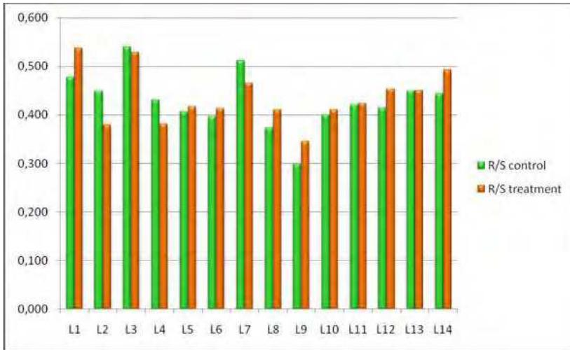
Fig. 6. Root to shoot ratio (dry weight) in maize landraces (L1-L14) at seedling stage
