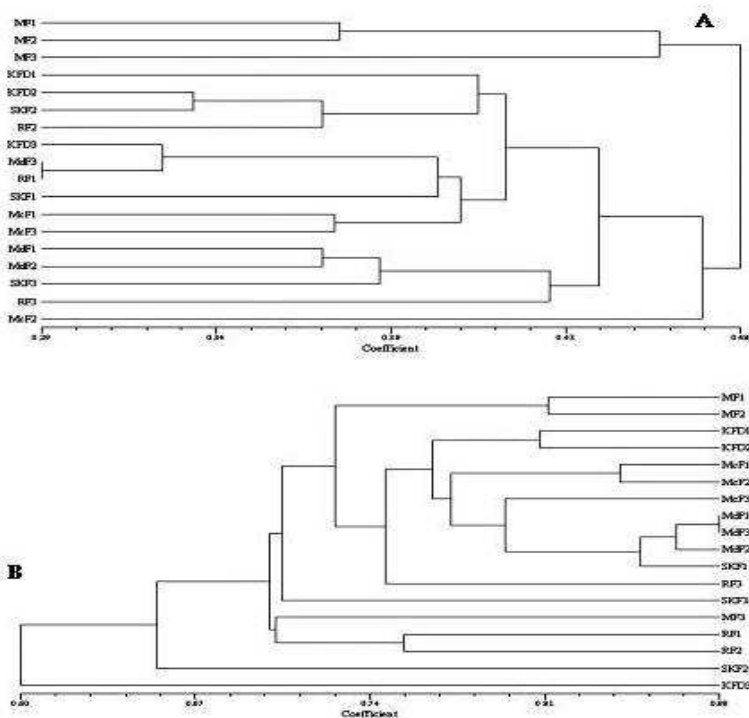
Fig. 3. Dendrograms of 18 maize populations (bulk population samples) constructed using UPGMA cluster analysis of A) Roger's distance values obtained by SSR analysis and B) Jaccard similarity values obtained by AFLP analysis. Abbreviations are the same as in Fig. 2.
