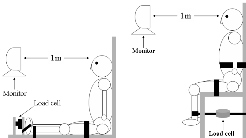
Fig. 3. Schematic drawing of the setup used for the isometric plantar flexion (left) and knee extension (right)
