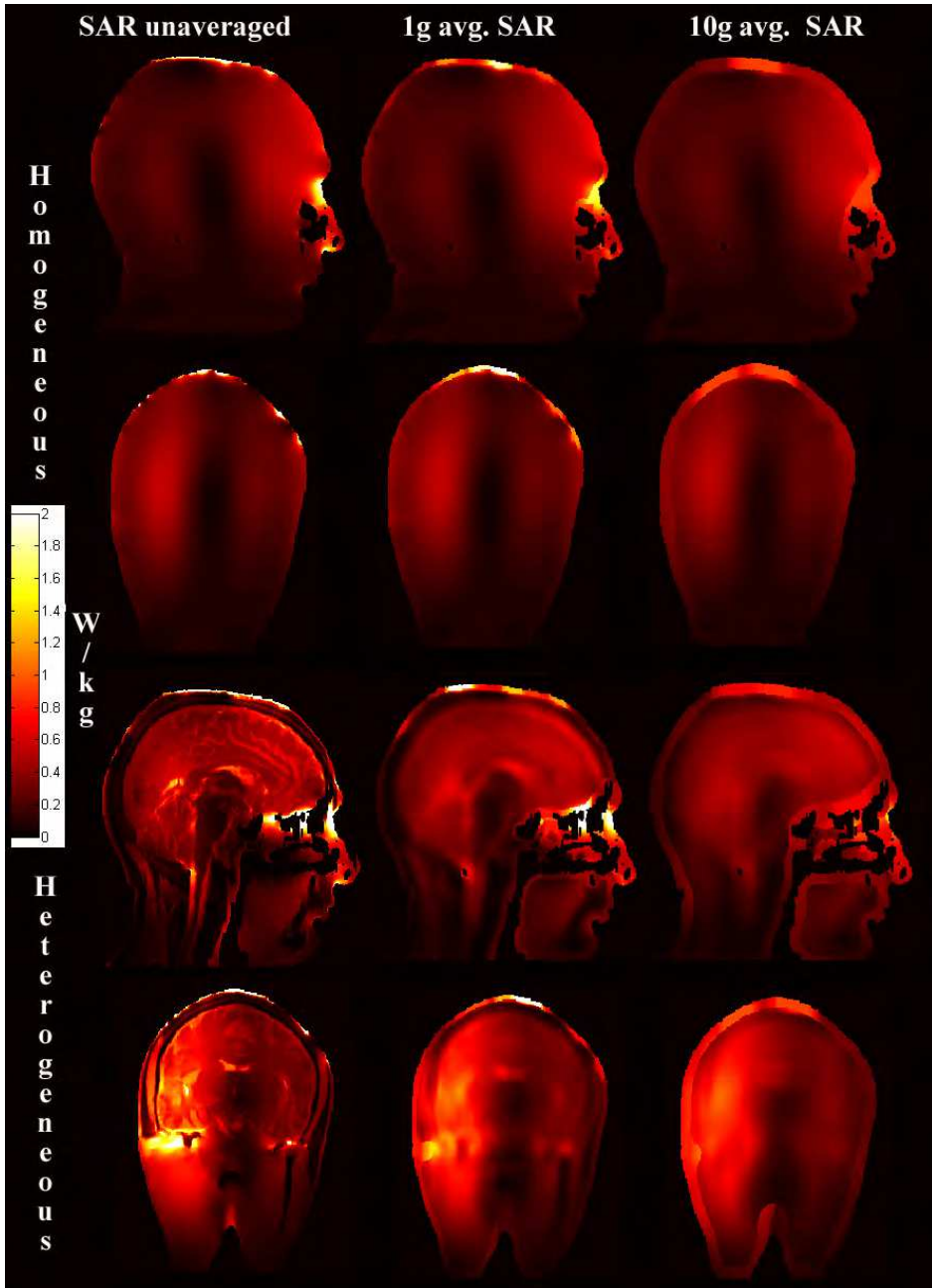
Fig. 5. Specific Absorption Rate (SAR) computed with an electrically homogeneous (top) and electrically heterogeneous (bottom head) model. Sagittal and coronal maps for SAR unaveraged, 1g-averaged and 10g-averaged SAR are shown.
