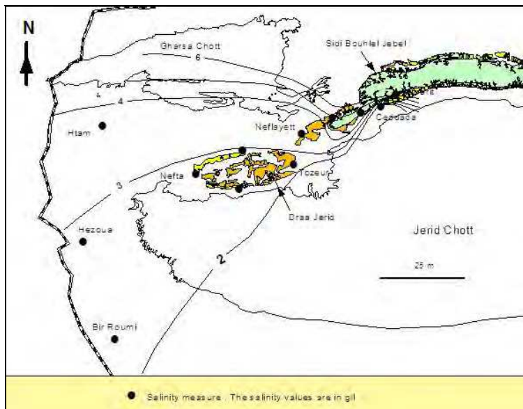
Fig. 7. Water salinity map of the Beglia aquifer (2008).
