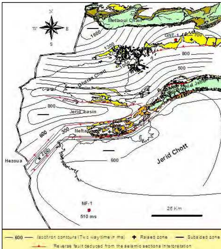
Fig. 10. Isochron map of the Beglia aquifer bottom.
