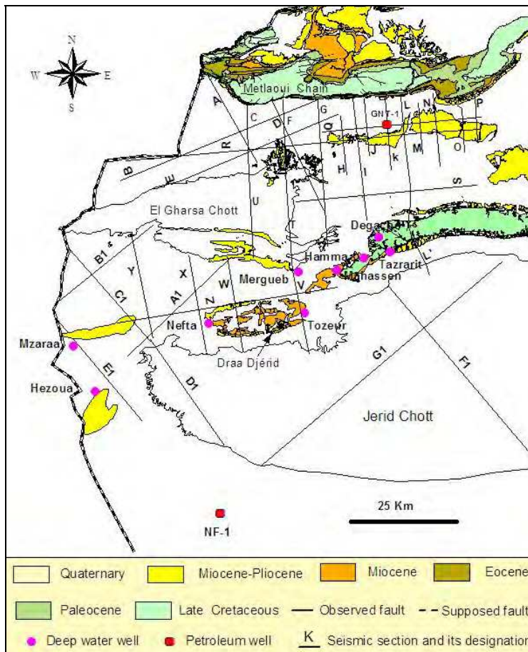
Fig. 8. Seismic profiles location.
