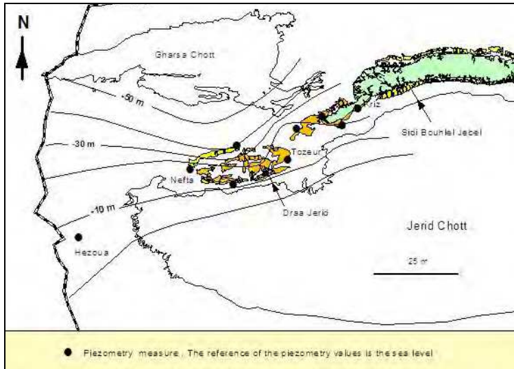
Fig. 6. Piezometric map of the Beglia aquifer (2008).
