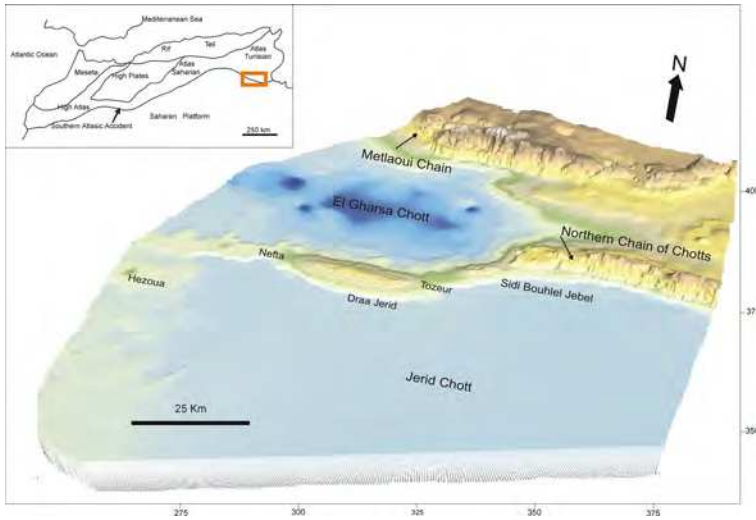
Fig. 2. Study area setting.
