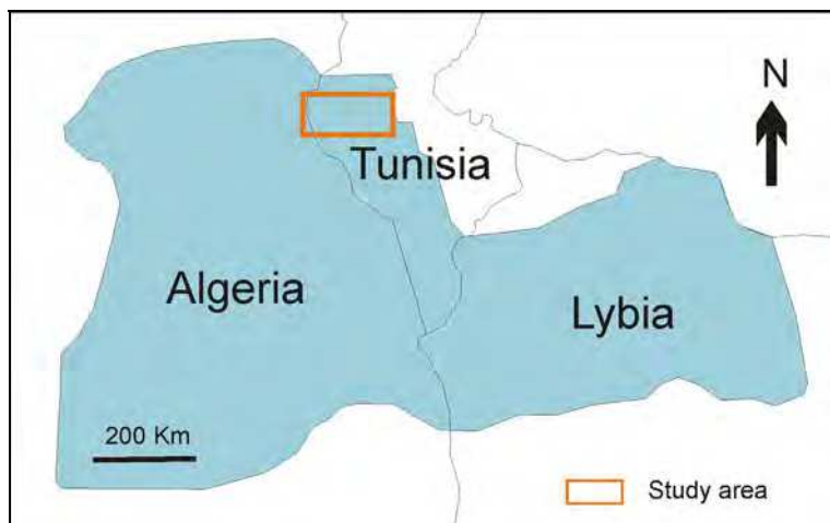
Fig. 1. Extent of the Complex Terminal aquifer (OSS, 2003, modified).
