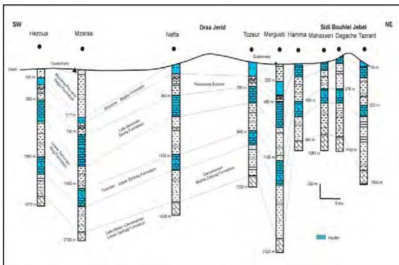
Fig. 5. Deep wells correlation.
