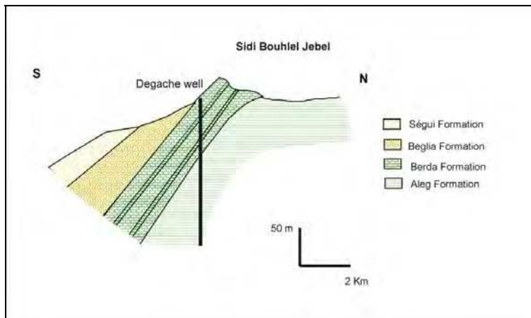
Fig. 4. Geological cross-section at Sidi Bouhlel Jebel.
