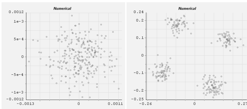
Fig. 21. Simulated constellation diagrams (a) without SOA, (b) with SOA compensator, L=500m , f_{subcarrier}=60GHz , modulation= 2048Mbps, 4QAM
