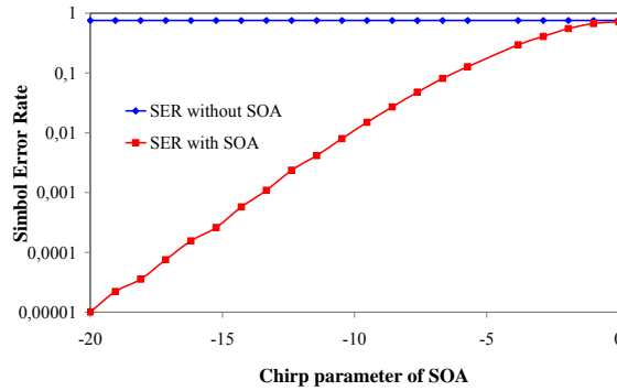
Fig. 20. Simulated Symbol Error Rate at frequency notch versus chirp parameter of SOA, L=500m , f_{subcarrier}=60GHz , modulation= 2048Mbps, 4QAM, without and with SOA
