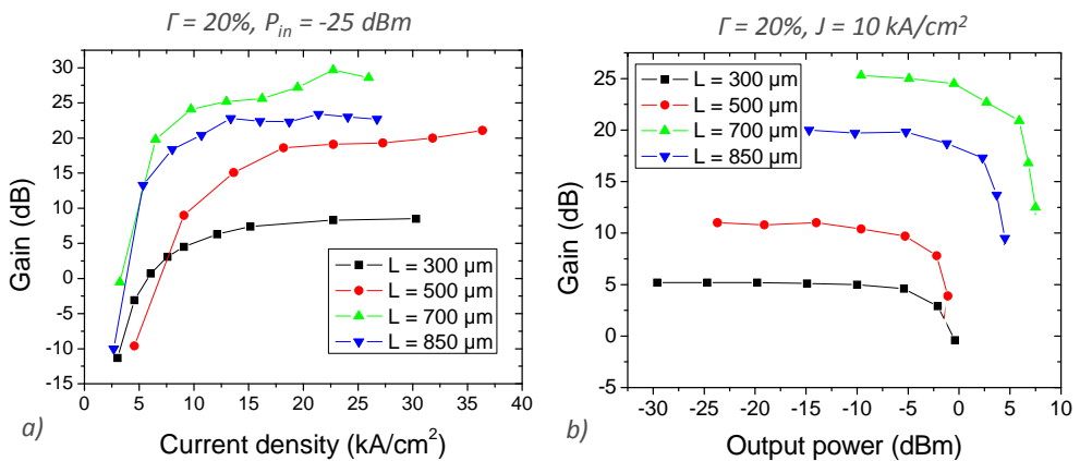
Fig. 6. Length effect on 20% optical confinement RSOA depending on the current density (a) and on the output power (b) for J = 10 kA/cm^2
