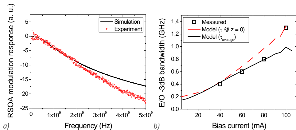
Fig. 12. RSOA (a) E/O modulation bandwidth versus frequency at I = 80 mA (b) -3 dB E/O modulation bandwidth versus bias current for 700µm of AZ
