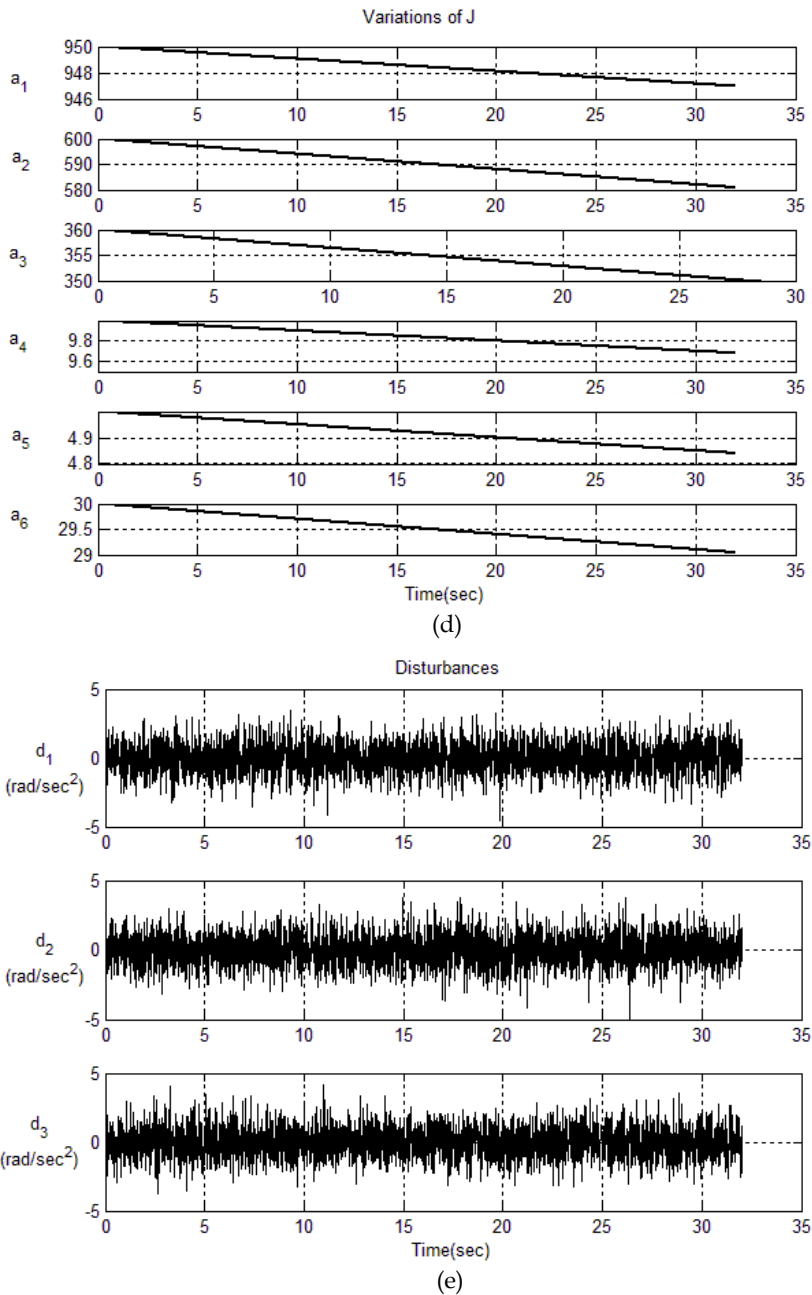
Fig. 5. Simulation results of (a) quaternion attitude tracking effects, (b) the convergence of sliding surface, (c) control torque inputs; (d) variations of J , and (e) real white Gaussian noises of power 1 dBW of the sliding-mode controller for spacecrafts.
