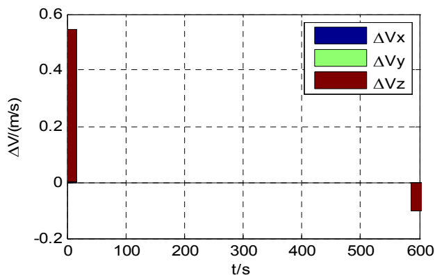
Fig. 13. Impulsive control input.
