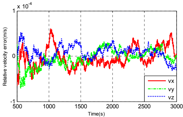
Fig. 7. Relative velocity estimation errors.
