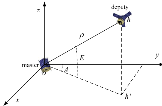
Fig. 4. Relative measurement geometry.
