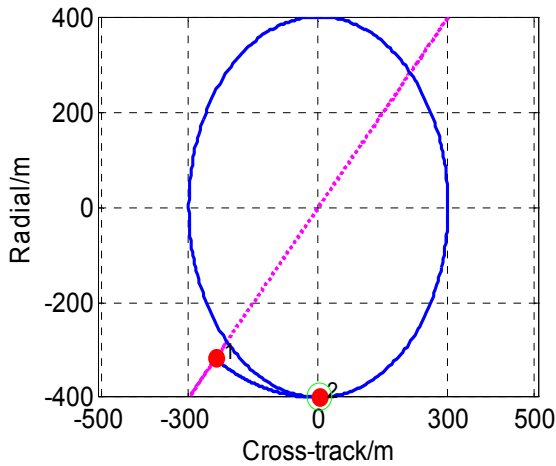
Fig. 15. Trajectory in the cross-track plane.
