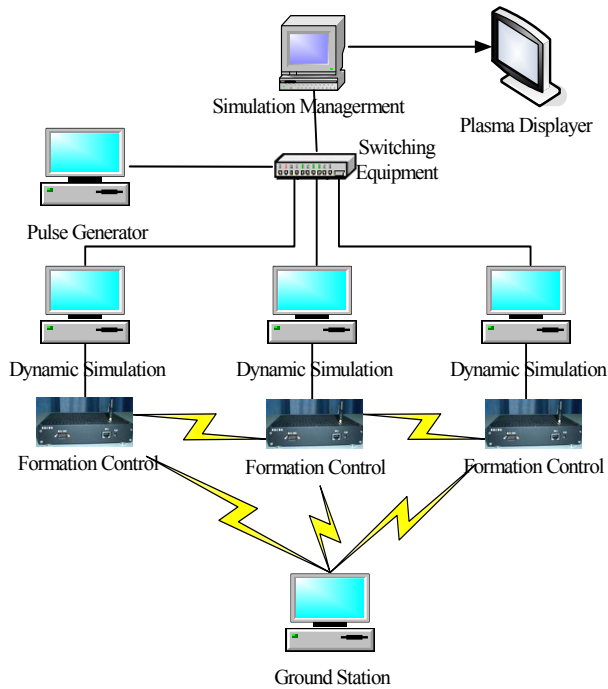
Fig. 17. Distributed architecture of the simulation system.
