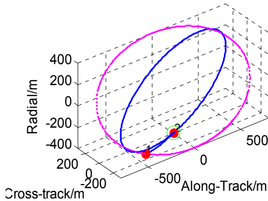
Fig. 14. Three-dimensional trajectory.
