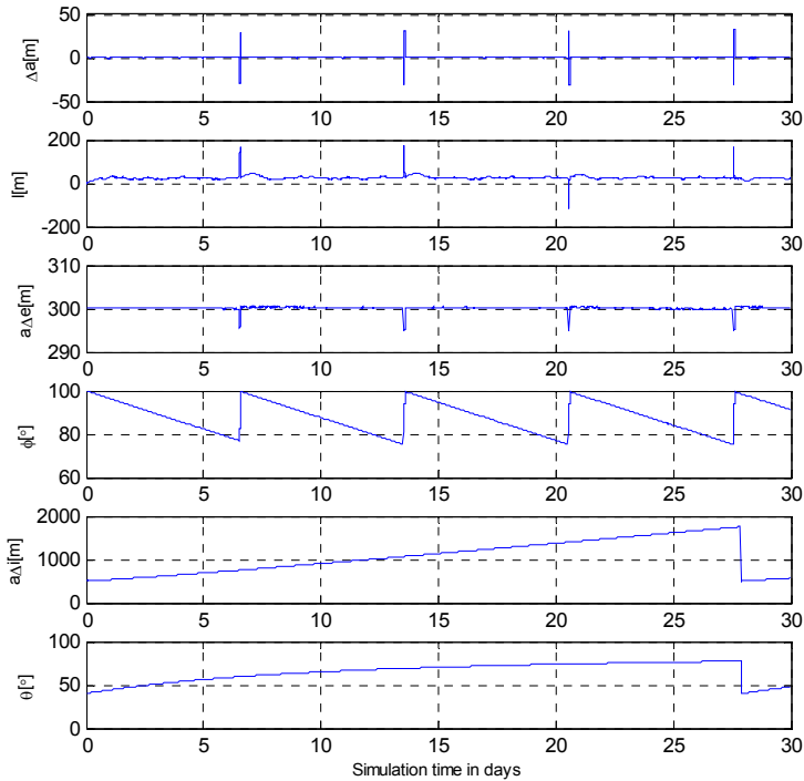
Fig. 19. The key results of formation keeping scenario.
