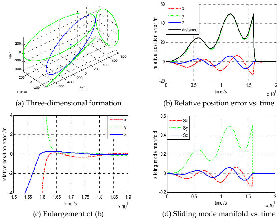
Fig. 9. Simulation results of formation keeping scenario.
