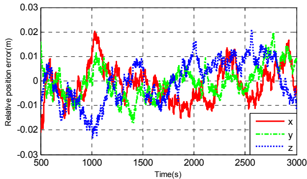
Fig. 6. Relative position estimation errors.
