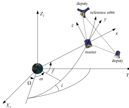
Fig. 1. J2000 inertial frame and Hill frame.
