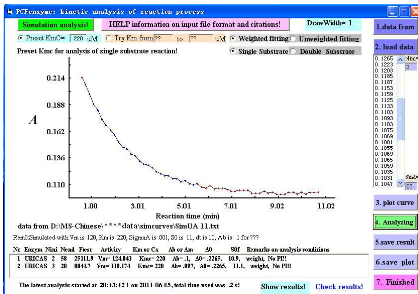
Fig. 11. Main window for the executable PCFenzyme
