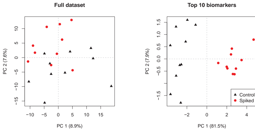
Fig. 2. PCA score plot (PC1 vs PC2) for the positive ion mode data set after standardization. In the left plot the principal components have been calculated on the full data set. In the right panel PCA analysis has been performed considering only the top 10 variables selected by a t -test.
