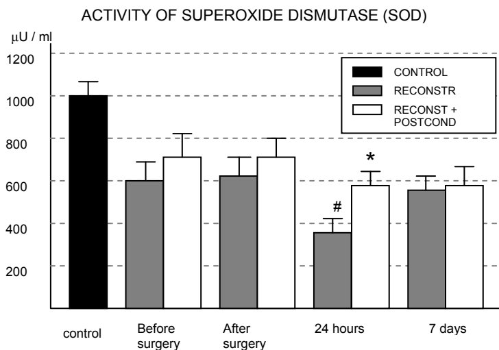
Fig. 4. Changes in blood superoxide dismutase activity during the examined perioperative period. (# p < 0.05 vs before surgery; * p < 0.05 vs non-conditioned group)
