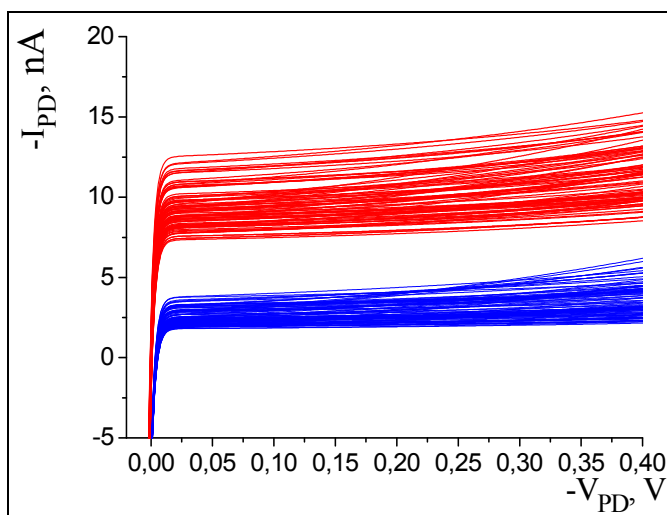
Fig. 11. A family of experimental current-voltage characteristics of Hg_{1-x}Cd_xTe photodiodes; “dark” characteristics are shown with blue lines, and characteristics measured under room-temperature radiation background with red lines are shown with red lines.
