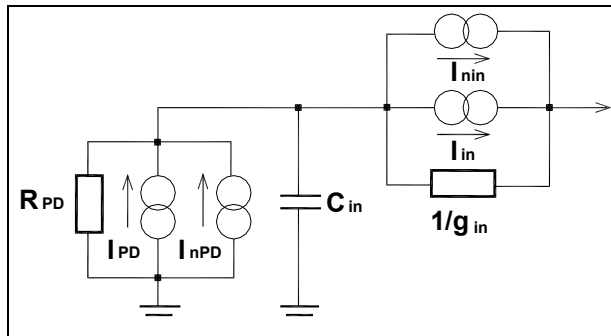
Fig. 2. The equivalent circuit of the photodiode channel of a hybrid IR FPA based on the system ‘photodiode – direct-injection readout circuits’. Here, I_{PD} is the current that flows through the photodiode, I_{nPD} is the noise current that flows through the photodiode, R_{PD} is the dynamic resistance of the photodiode, I_{in} is the current integrated under the storage gate of the readout circuit, I_{nin} is the noise current integrated under the storage gate, and C_{in} is the capacitance of the input direct injection.
