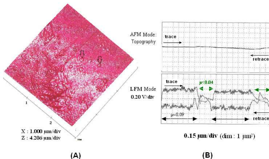
Fig. 8. Annealed fiber E41: (A) topographic image; (B) scope-mode forward and backward scanned AFM and LFM signals.
