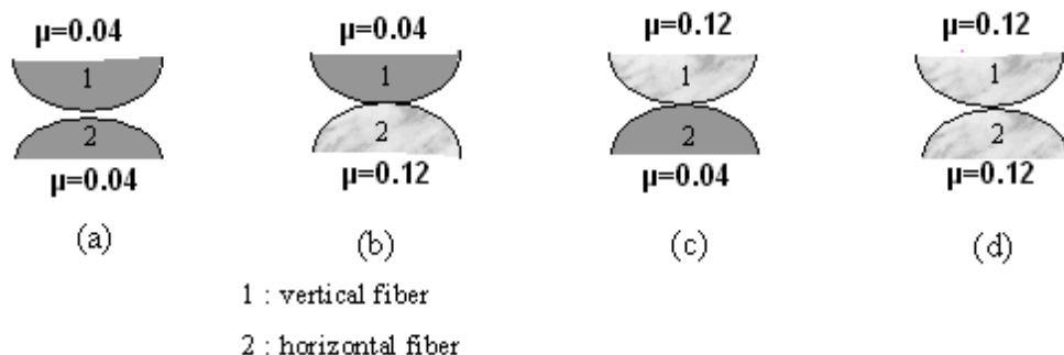
Fig. 10. Modelling the different contacts possible during fiber-fiber friction of the sized fiber A (the friction coefficients are those evaluated by LFM)
