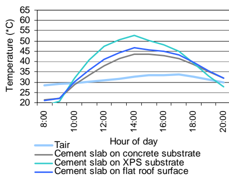
Fig. 2. Short-scale preliminary study. Mean daily temperature fluctuation.
