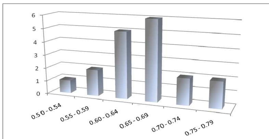
Fig. 7. Frequency of occurrence of Hurst exponents H.
