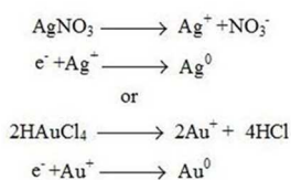
Scheme 1. Ascorbic acid reduction mechanism of gold and silver ions to obtain \text{Ag}^0 and \text{Au}^0 nps.
