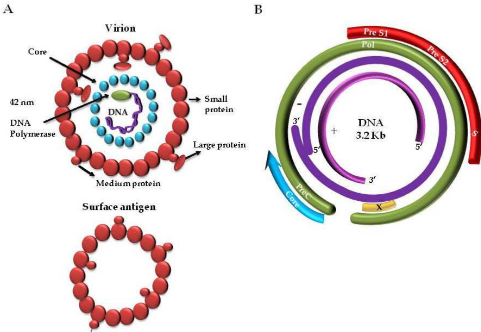
Fig. 3. HBV virion and genome organization. A. Enveloped virion of 42 nm. The 3 forms of HBV surface antigen (small, medium and large) are embedded in the lipid envelop which covers the core which interacts with the partially double stranded DNA, which is covalently linked to the polymerase. Cellular heat shock proteins inside the virion are not shown. In addition to the virion, HBV surface antigen empty particles are secreted both as spherical or cylindrical particles. B. The DNA genome and the 4 ORFs are shown, describing the compact nature of this genome.
