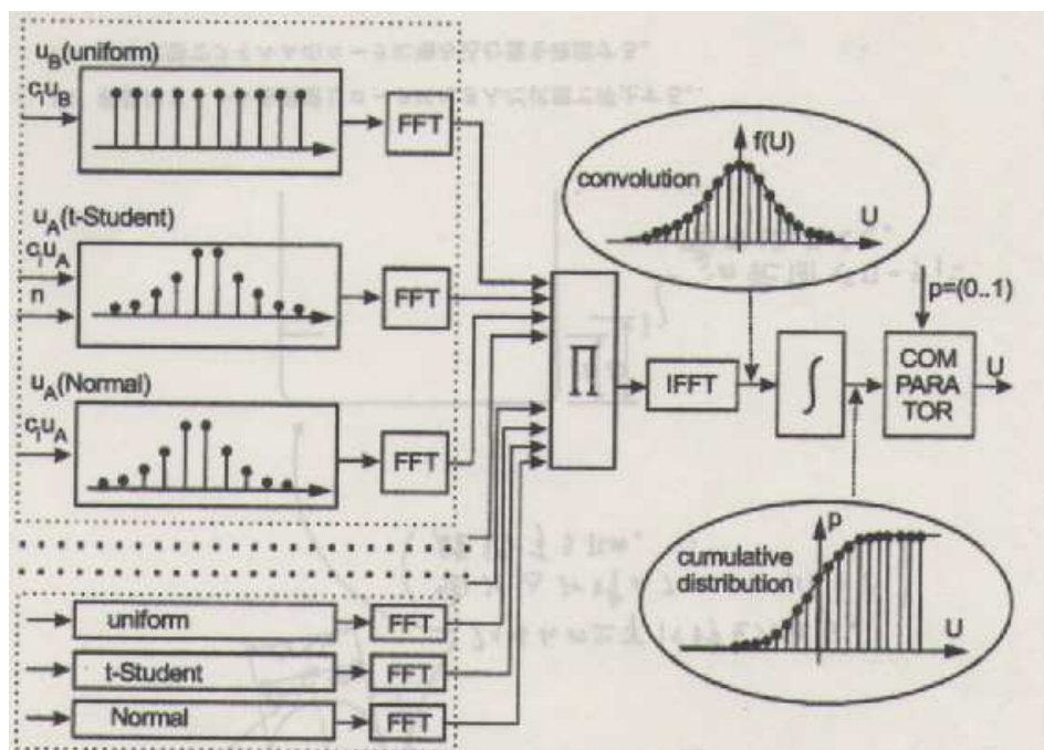
Fig. 3. MCM of EDA in 2002 by rule of NIST
