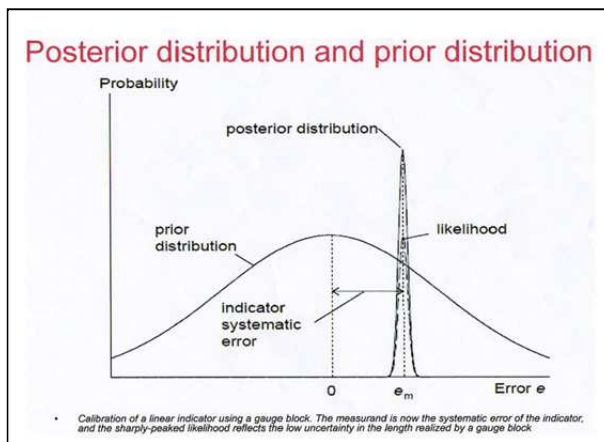
Fig. 2. Posterior distribution and prior distribution
