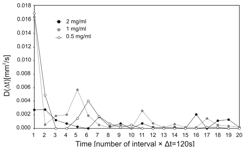
Fig. 6. The diffusion coefficient in water solution of liposomes measured in the given time interval \Delta t by the laser interferometric system.
